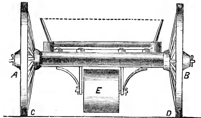
ROAD PROTECTOR, 1796.
